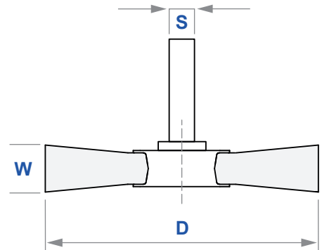
Mounted Wire Wheel 6mm Shank
